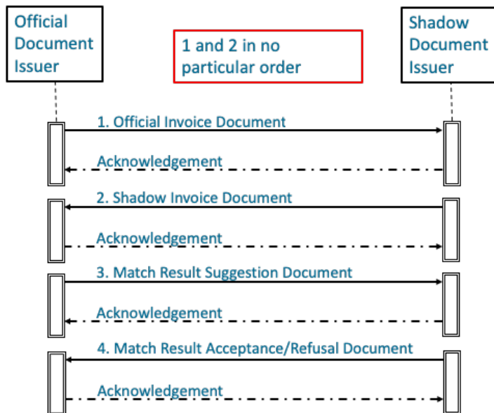
Figure 3: Invoice Matching Dialogue
